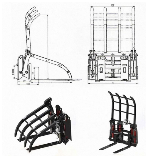
Structural line diagram
