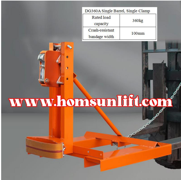
DG360A Single Barrel, Single Clamp
