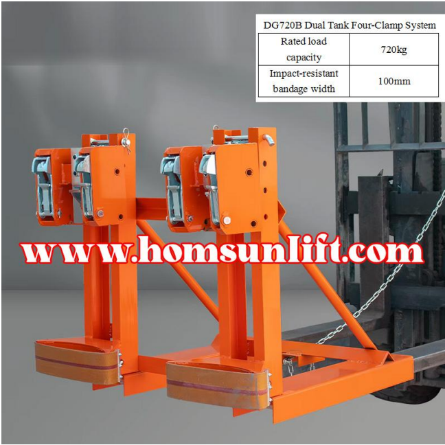
DG720B Dual Tank Four-Clamp System
